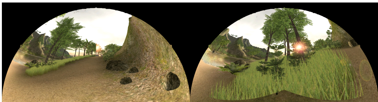
Figure 6. Two artifacts arising from effects created in a postprocessing phase or those with a camera direction dependence. Left: sun effects at the seam of the left and right cube face. Right: grass planes on the bottom face parallel to camera view direction.
